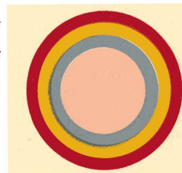
Etheric Structure of Earth:
