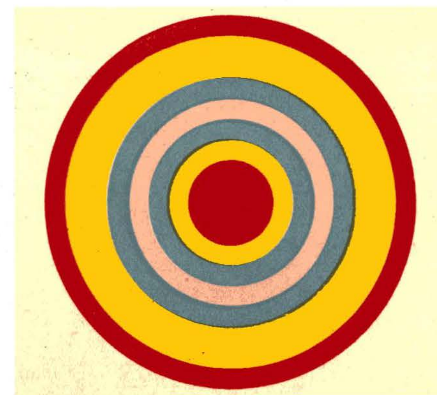
Earth with its Interior (represented as differentiated)
