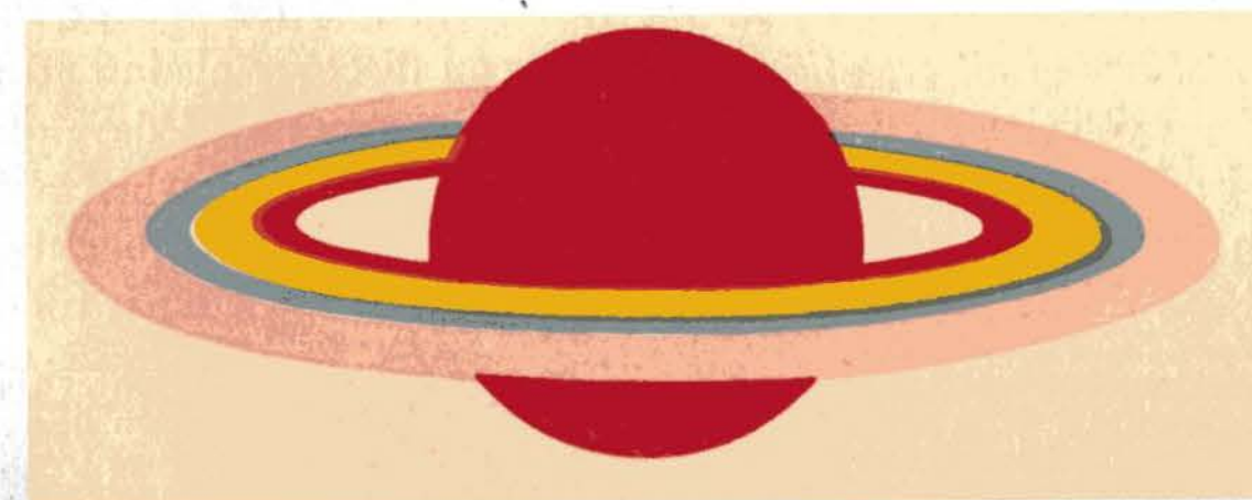
Etheric Structure of Saturn:
