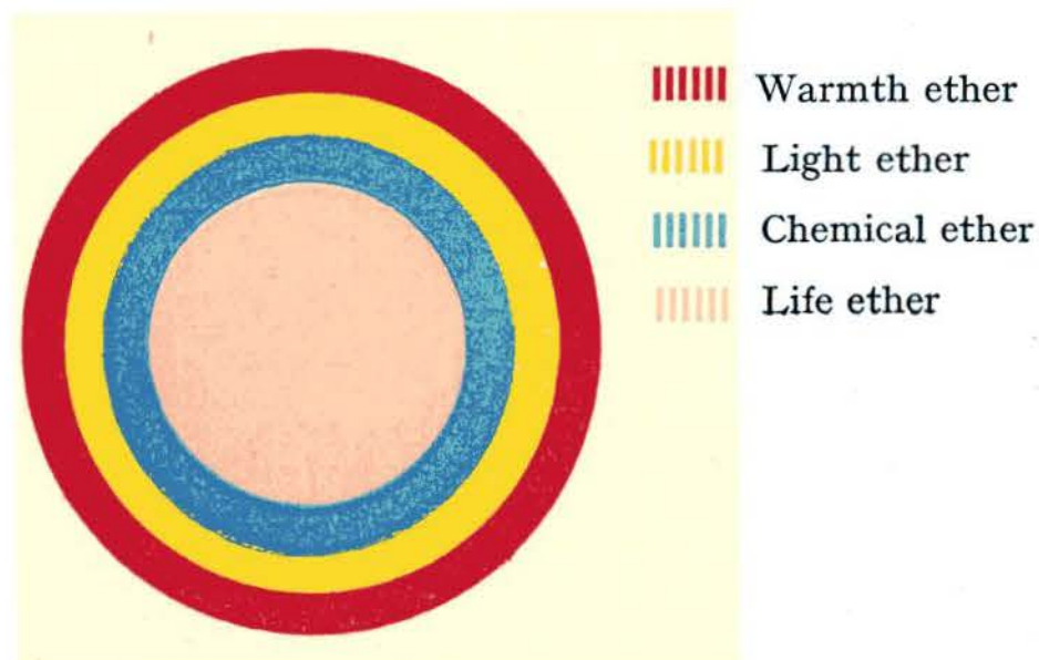
Basic structure of the earth.
