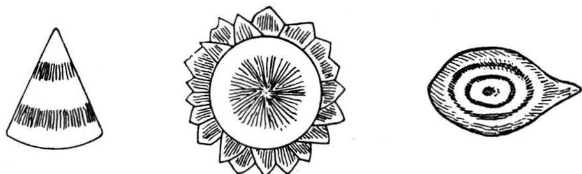
Hail stones (after Professor Trabert)
