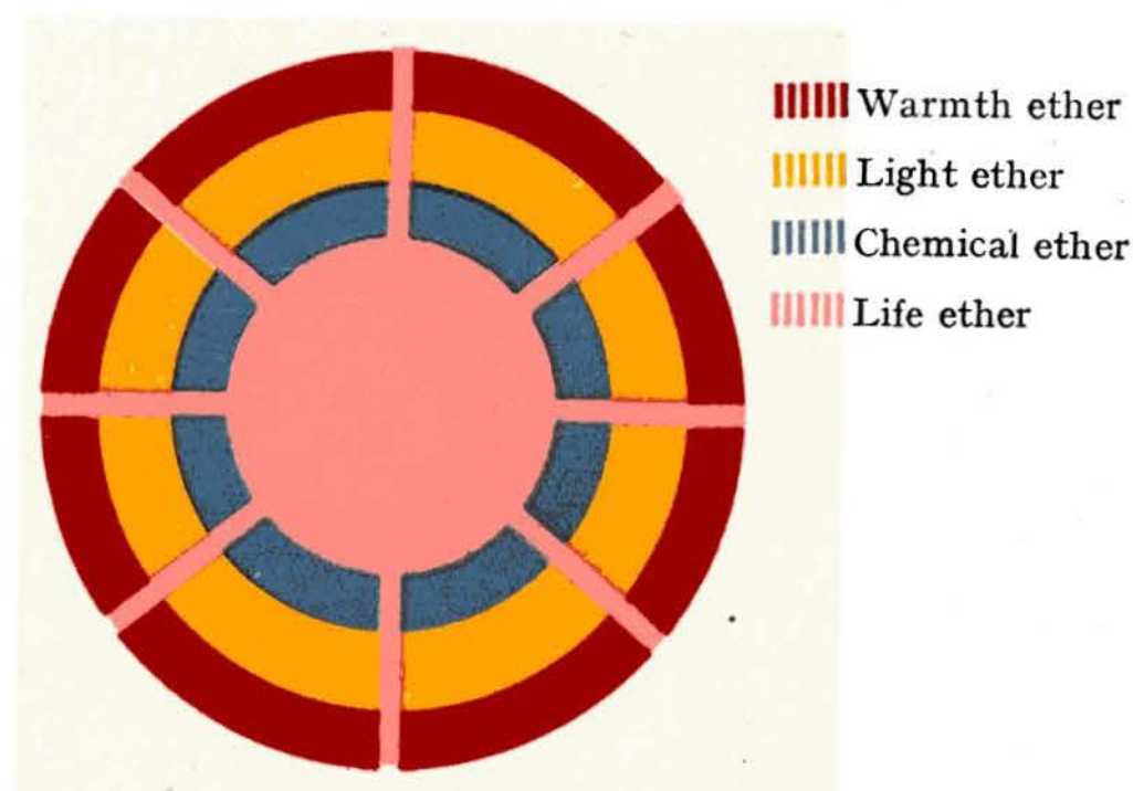
Picture of the earth organism, and likewise of the substance unit.
