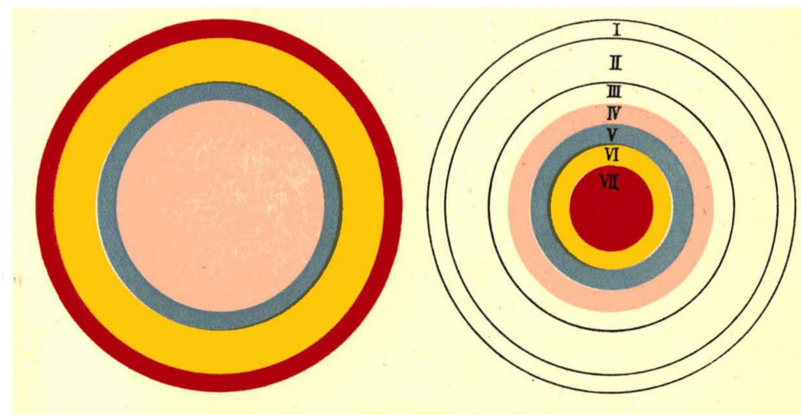
Earth with its Interior (represented as differentiated)
