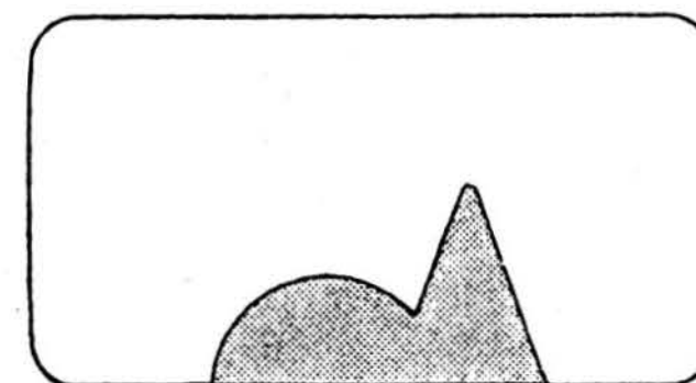
Half-moon form. Triangular form.
